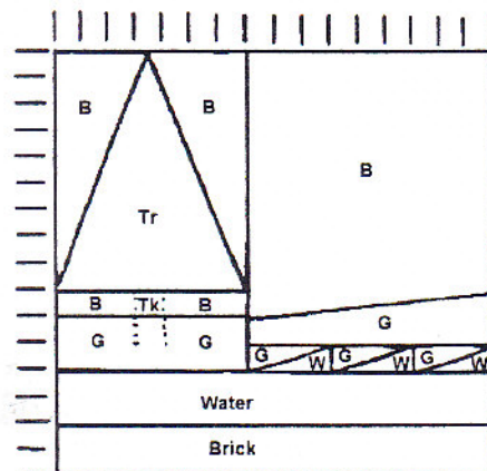
Figure 2: Piecing Diagram
